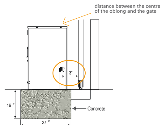
Dimensions (inches)
